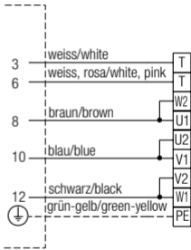
Motor \Delta
