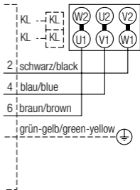
Motor \Delta
